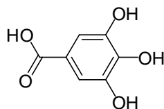
Fig. 1: Structure of Gallic acid.
