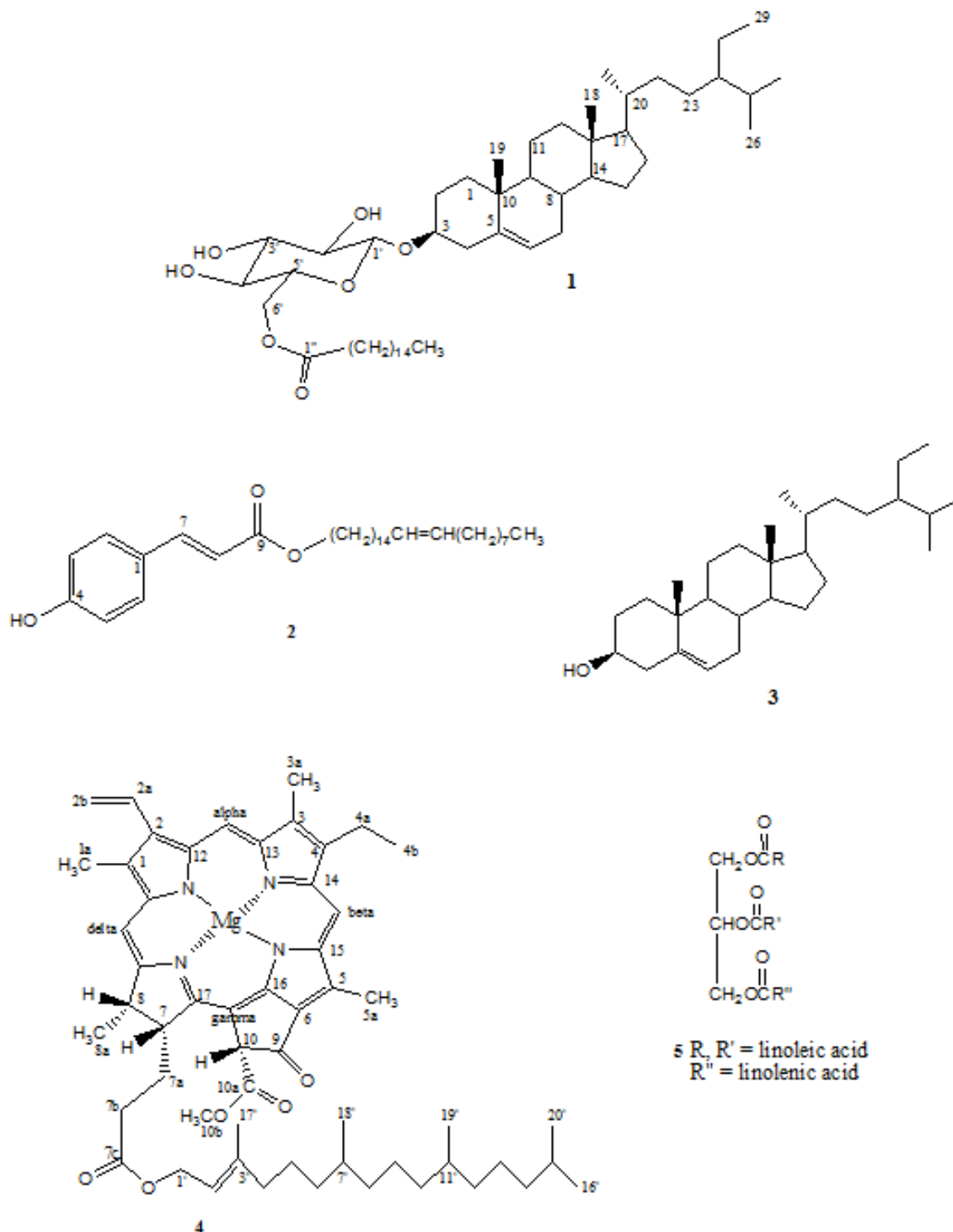
Fig. 1: Chemical structures of \beta -Sitosteryl-3 \beta -glucopyranoside-6'- O -palmitate ( 1 ), nervonyl 4-hydroxy- trans -cinnamate ester ( 2 ), \beta -sitosterol ( 3 ), chlorophyll a ( 4 ), and 1,2-dilinoleoyl-3-linolenoylglycerol ( 5 ) from C. dichotoma .
